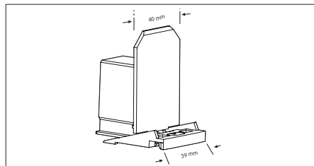
PRV +S H0 Without front
