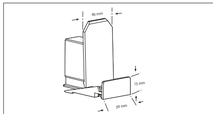
PRV +S H15 With front 15 mm
