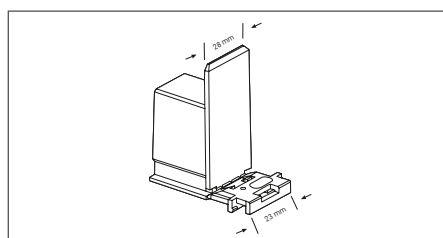
PRV +S SLIM H0 Without front
