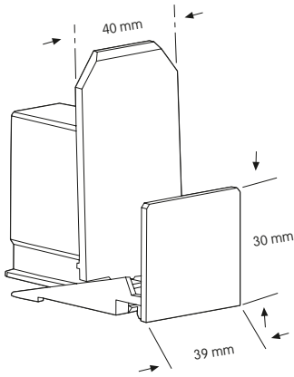
PRV +S H30 With front 30 mm
