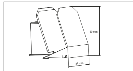
PRV +S H60 With front 60 mm, 20° inclined
