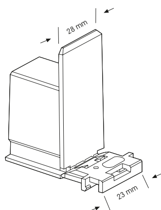
PRV +S SLIM H0 Without front
