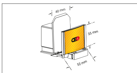
PRV H35 With front 35 mm
